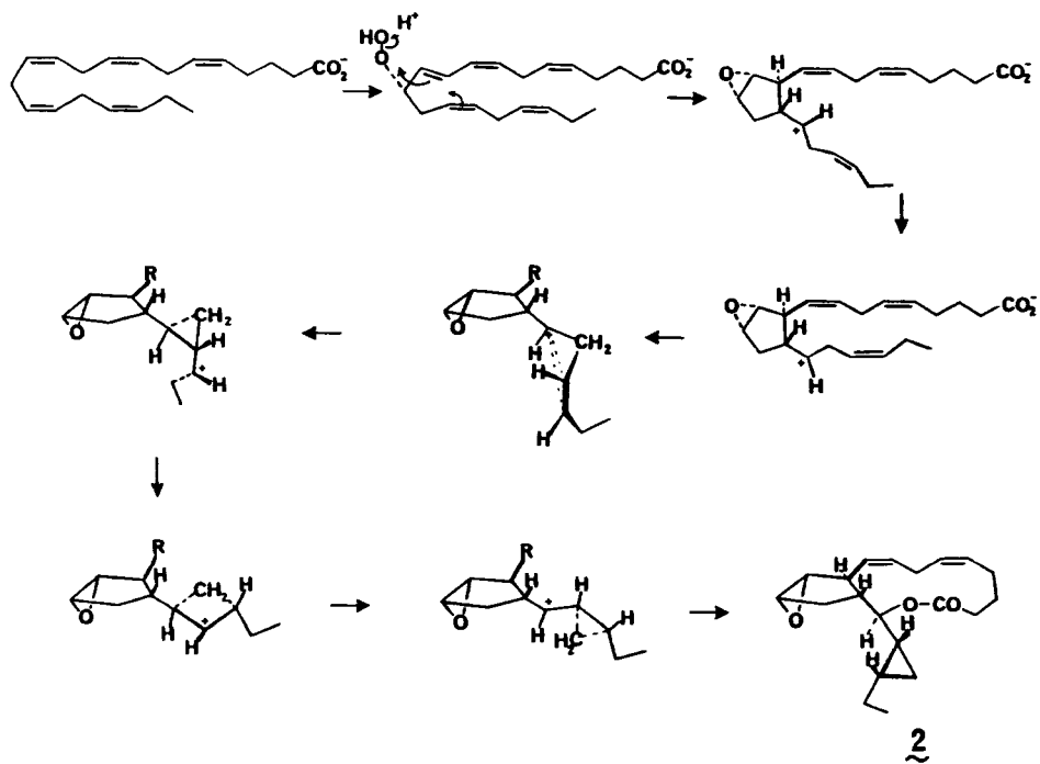
PROPOSED BIOSYNTHESIS OF HYBRIDALACTONE
