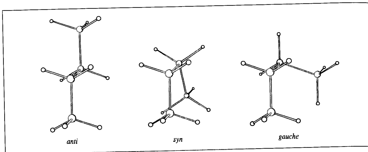
Fig 2.19. syn, anti and gauche conformations of butane (C-C-C-C torsion angles 0^\circ , 180^\circ and \pm 60^\circ respectively).
