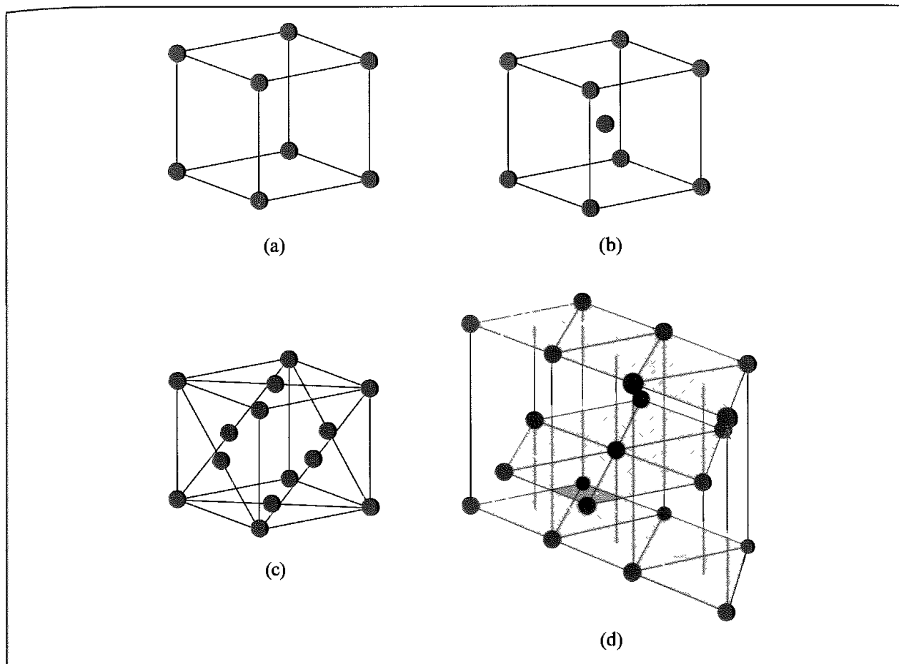
Fig. 3.8 Some basic Bravais lattices (a) simple cubic, (b) body-centred cubic, (c) face-centred cubic and (d) simple hexagonal close-packed (Figure adapted in part from Ashcroft N W and Mermin N D 1976. Solid State Physics New York, Holt, Rinehart and Winston.)
