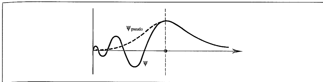
Fig. 3.22 Schematic representation of a pseudopotential (Figure adapted from Payne M C, M P Teter, D C Allan, R A Arias and D J Joannopoulos 1992 Iterative Minimisation Techniques for Ab initio Total-Energy Calculations: Molecular Dynamics and Conjugate Gradients . Reviews of Modern Physics 64 1045-1097.)
