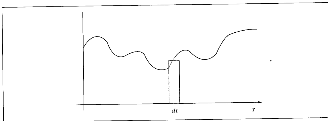
Fig 3.6 Schematic representation of the way in which the local density approximation assumes that the electron density within a volume element dr surrounding a point \mathbf{r} is assumed to be constant.
