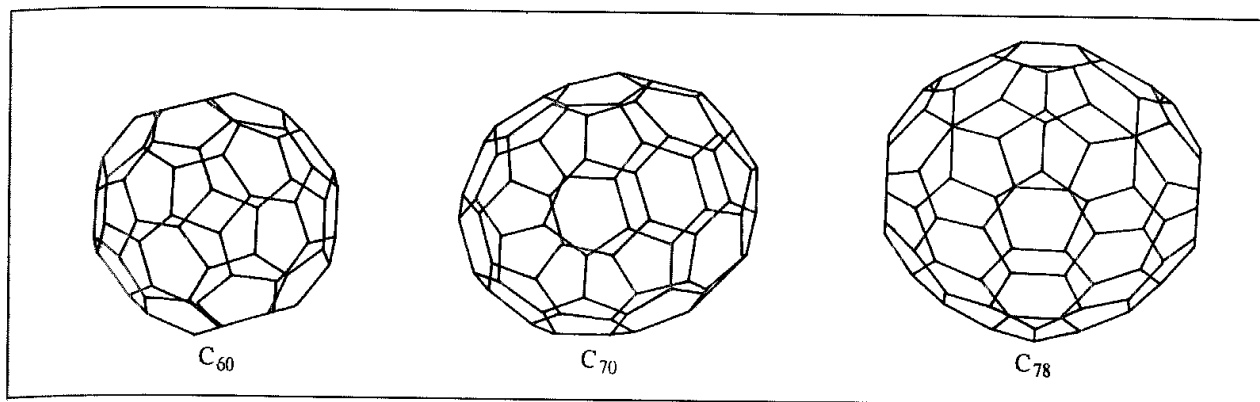
Fig 2.22 Three fullerenes, C 60 , C 70 and C 78 .
