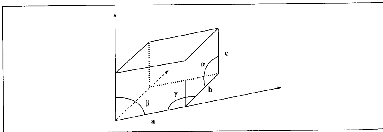
Fig. 3.7. The six parameters \mathbf{a} , \mathbf{b} , \mathbf{c} , \alpha , \beta , \gamma which characterise the unit cell.
