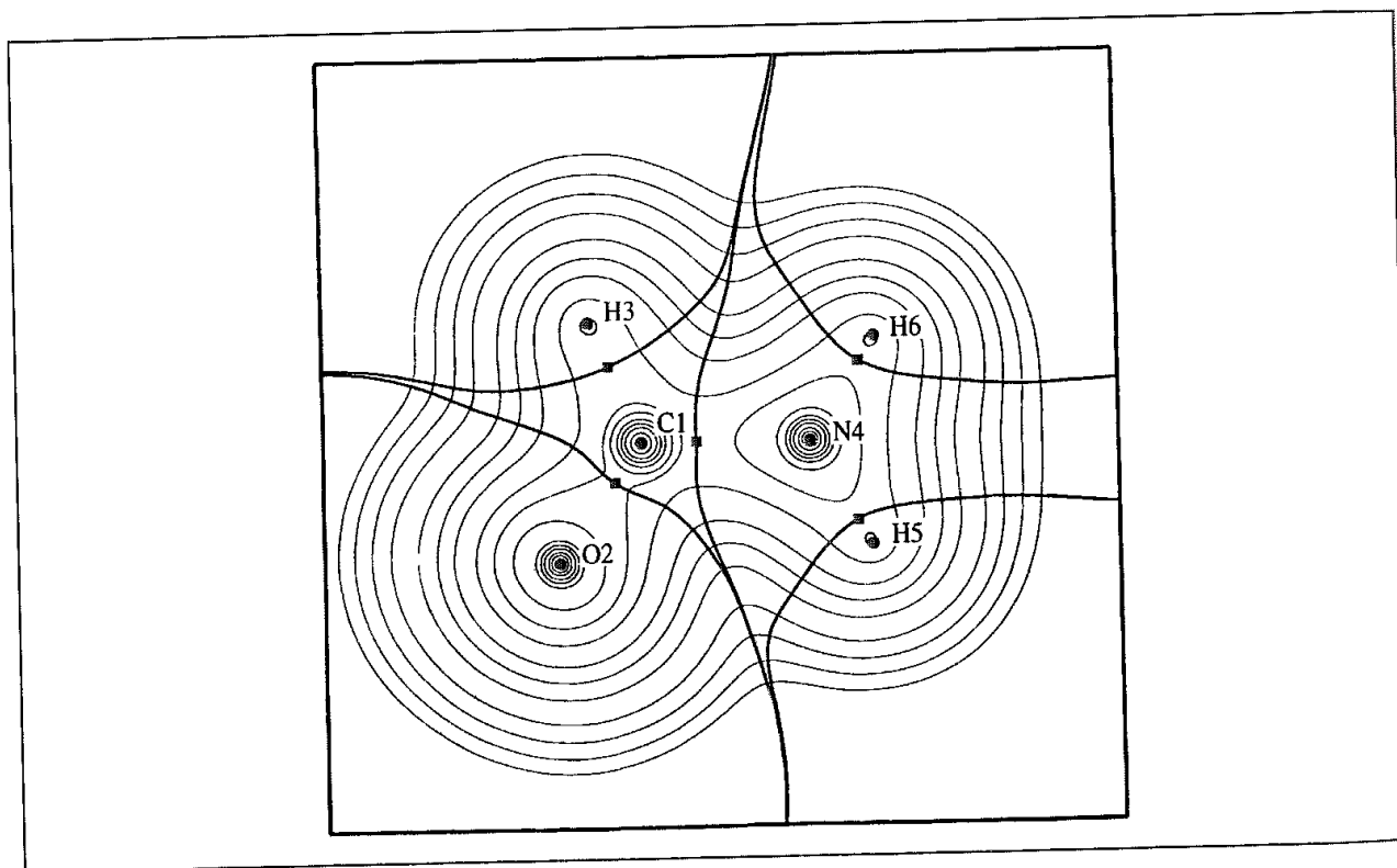
Fig 2 16· Partitioning the electron density in formamide
