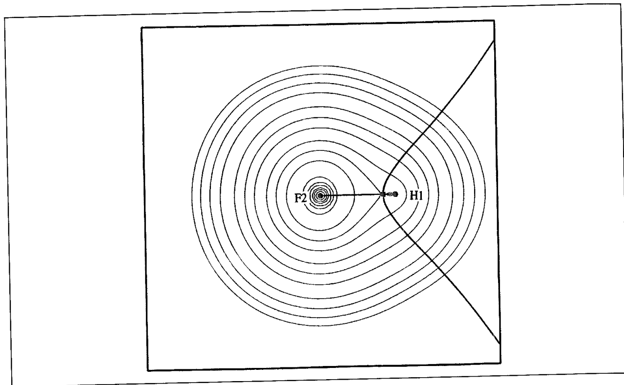
Fig 2 15· Partitioning the electron density in hydrogen fluoride
