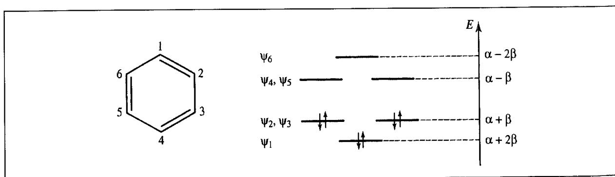
Fig 2.21: Benzene and its Hückel molecular orbitals.
