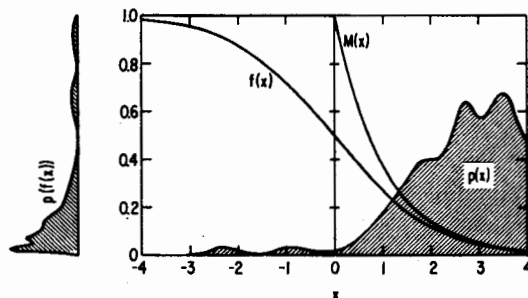
FIG. 1. The Fermi function, f(x) = 1/[1 + \exp(+x)] , and the Metropolis function, M(x) = \min\{1, \exp(-x)\} , are shown along with a typical probability density, p(x) , for their argument. Plotted on the left is a typical probability density for values of the Fermi function.
