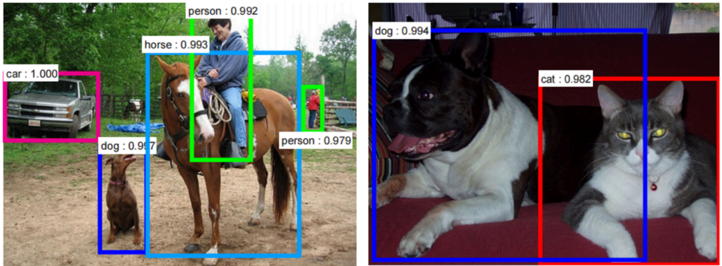
Figure 2: Source [2 ( https://arxiv.org/pdf/1506.01497v3.pdf )]
