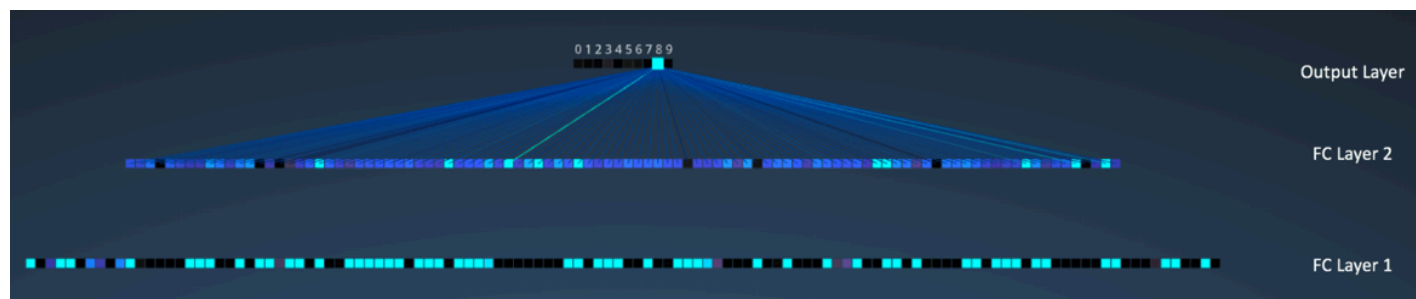
Figure 20: Visualizing the Fully Connected Layers. Source [13] ( http://scs.ryerson.ca/~aharley/vis/conv/flat.html )
