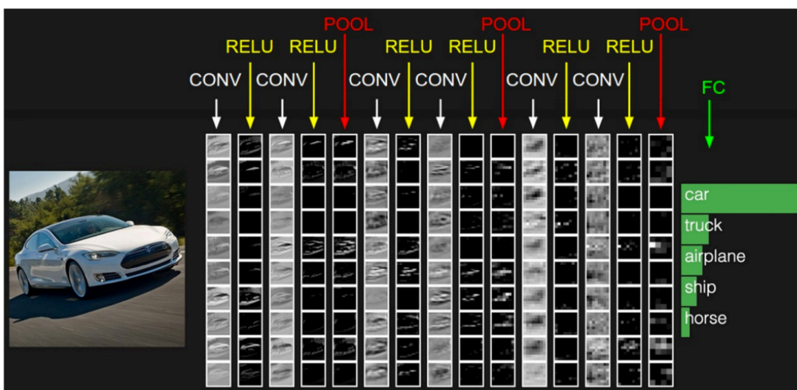
Figure 16: Source [4 ( http://cs231n.github.io/convolutional-networks/ )]
