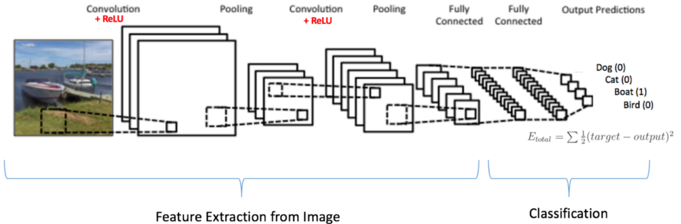
Figure 15: Training the ConvNet
