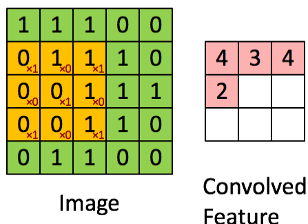
Figure 5: The Convolution operation. The output matrix is called Convolved Feature or Feature Map. Source [7 ( http://deeplearning.stanford.edu/wiki/index.php/Feature_extraction_using_convolution )]
