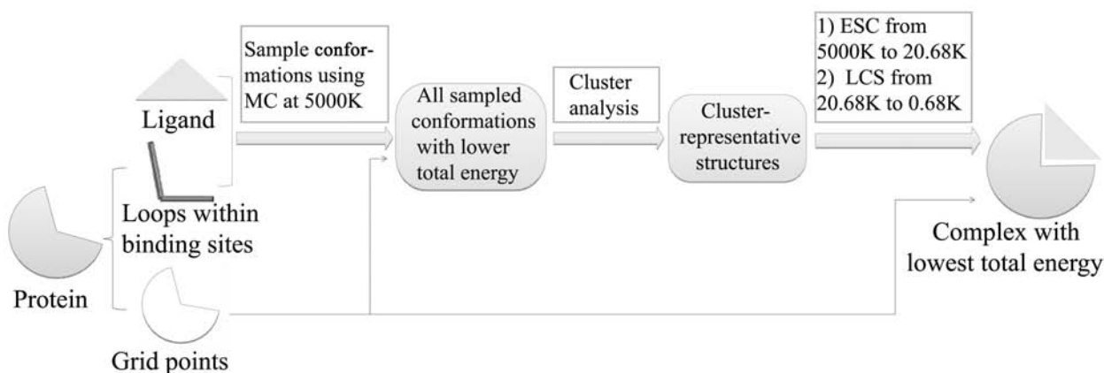
Fig. (4). Flowchart of local move Monte Carlo (LMMC) loop sampling approach for protein-ligand docking. Abbreviate: MC: Monte Carlo; ESC: Exponential Cooling Schedule; LCS: Linear Cooling Schedule.
