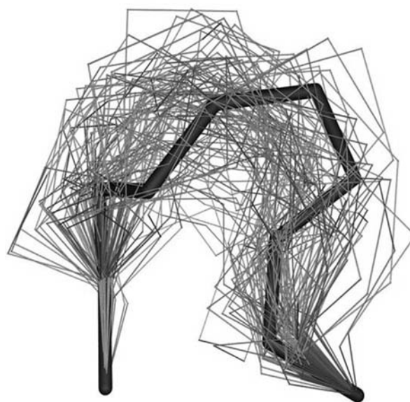
Fig. (3). Loop Structure of 2act (198-205) produced by the local move MC method at 5000K and followed by clustering to generate 100 representative conformations. Black stick represents the crystal loop structure, and gray wires represent the 100 representative loop conformations.
