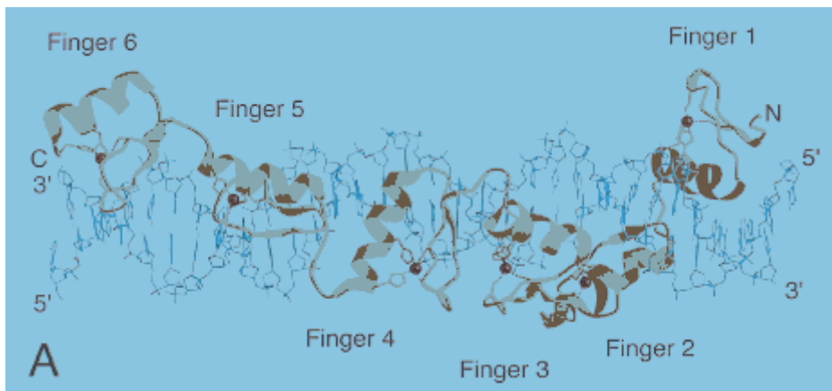
Structure of TFIIIA Fingers 1-6 bound to DNA.
