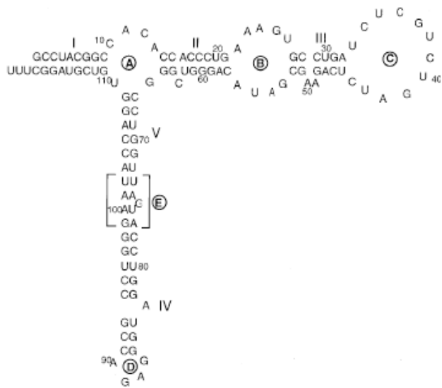
Secondary structure of 5S rRNA.
